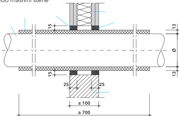
Detail N -
